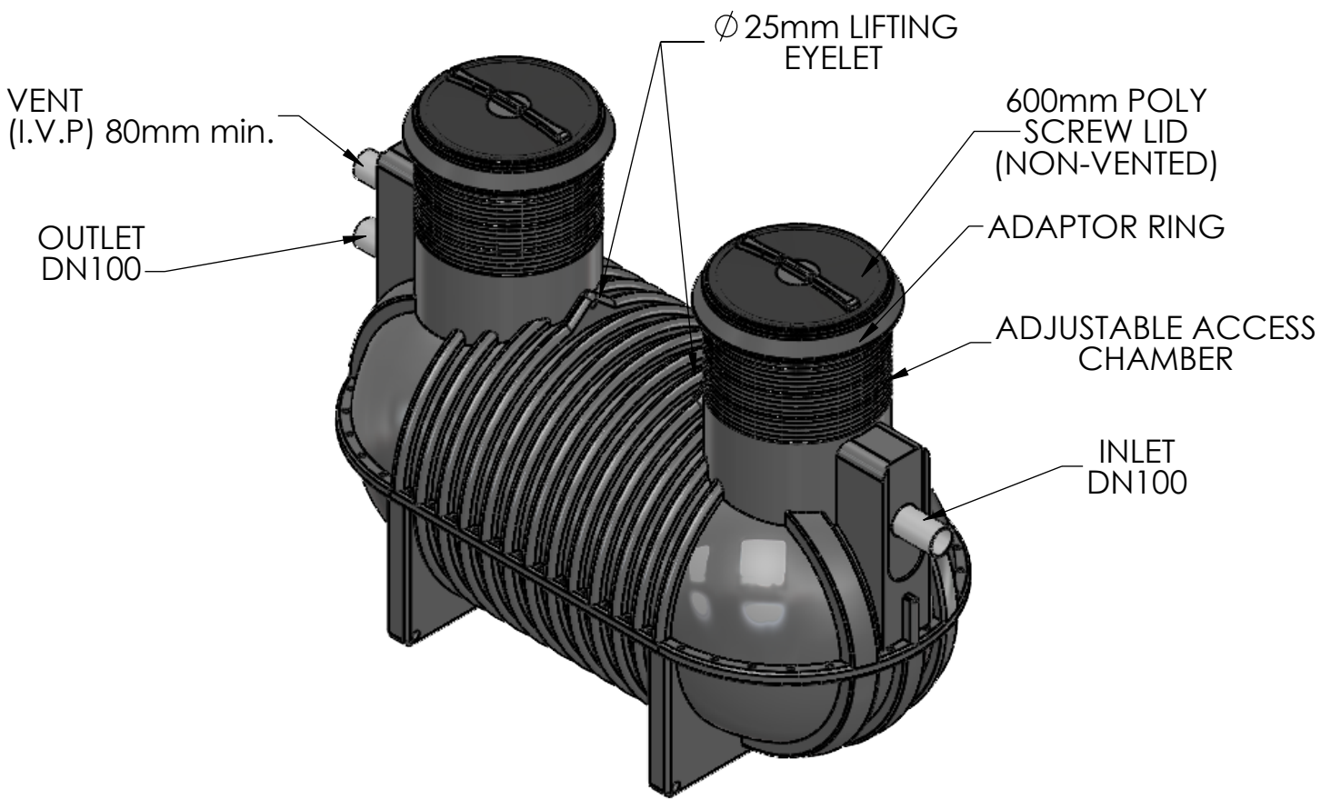
ISOMETRIC VIEW
