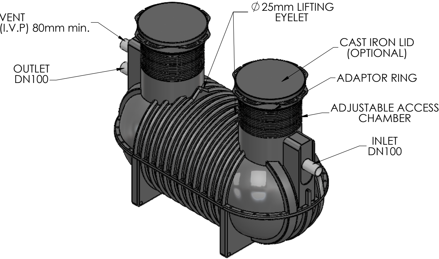
ISOMETRIC VIEW
