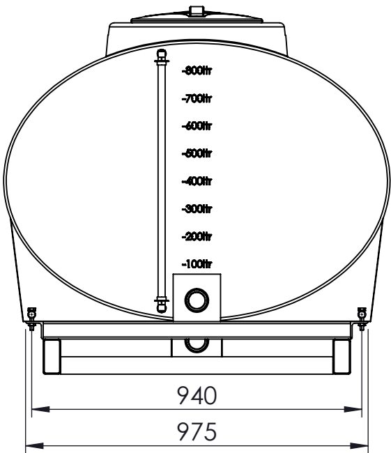
3 O'CLOCK VIEW
