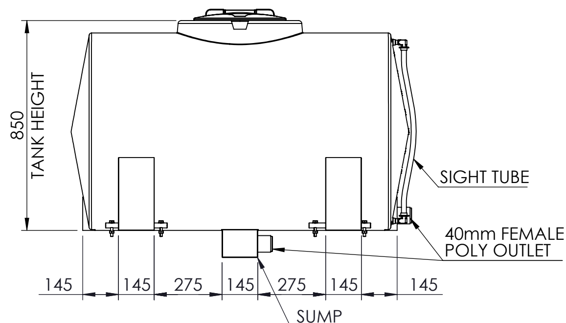
6 O'CLOCK VIEW
