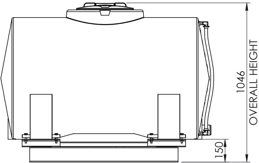
6 O'CLOCK VIEW
