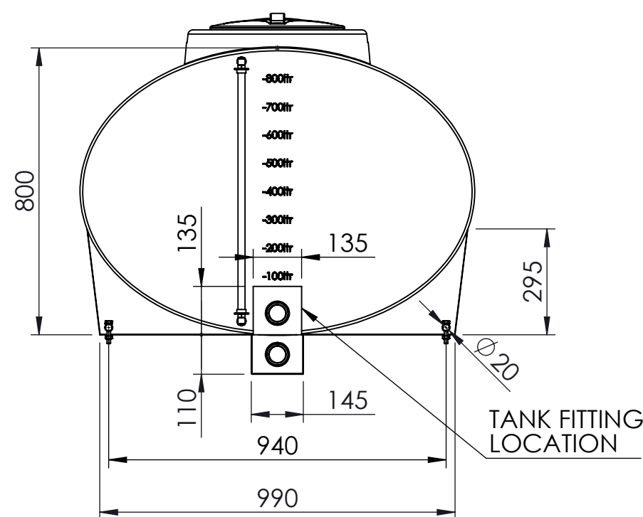
3 O'CLOCK VIEW
