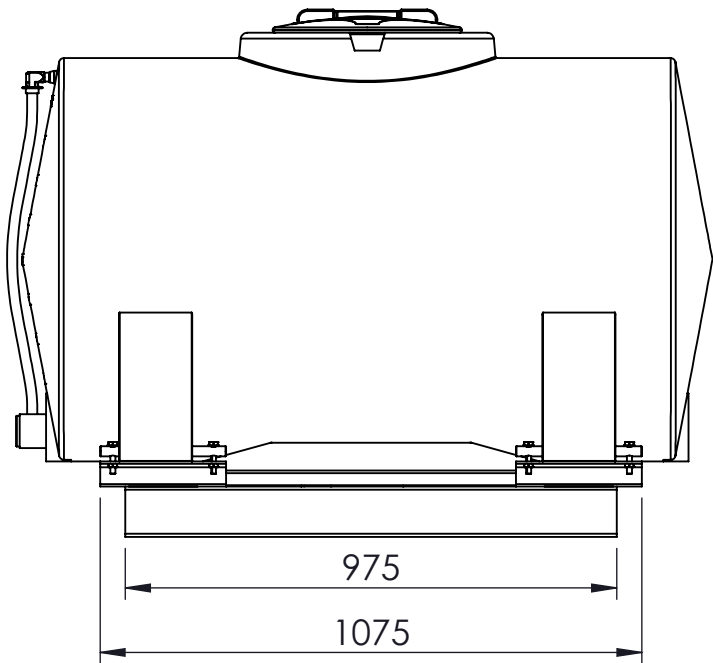
12 O'CLOCK VIEW
