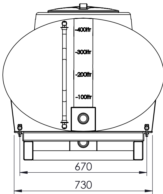
3 O'CLOCK VIEW
