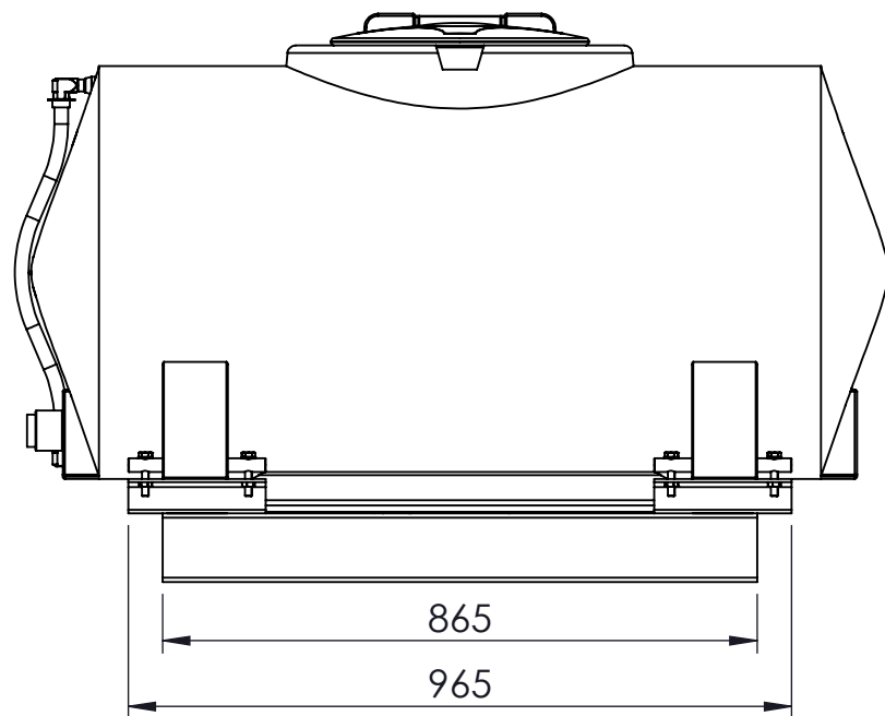
12 O'CLOCK VIEW
