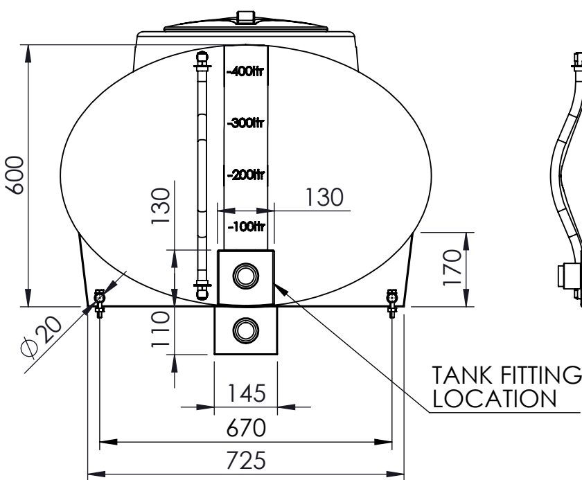
3 O'CLOCK VIEW
