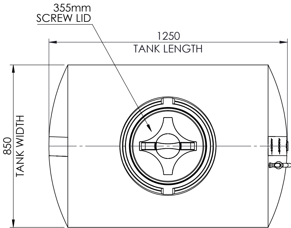
TOP VIEW
