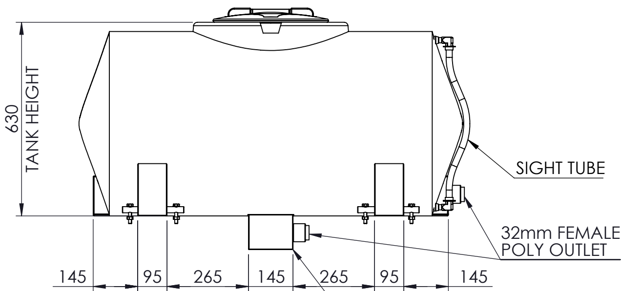
6 O'CLOCK VIEW
