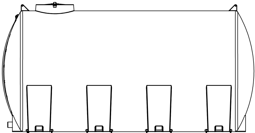
12 O'CLOCK VIEW
