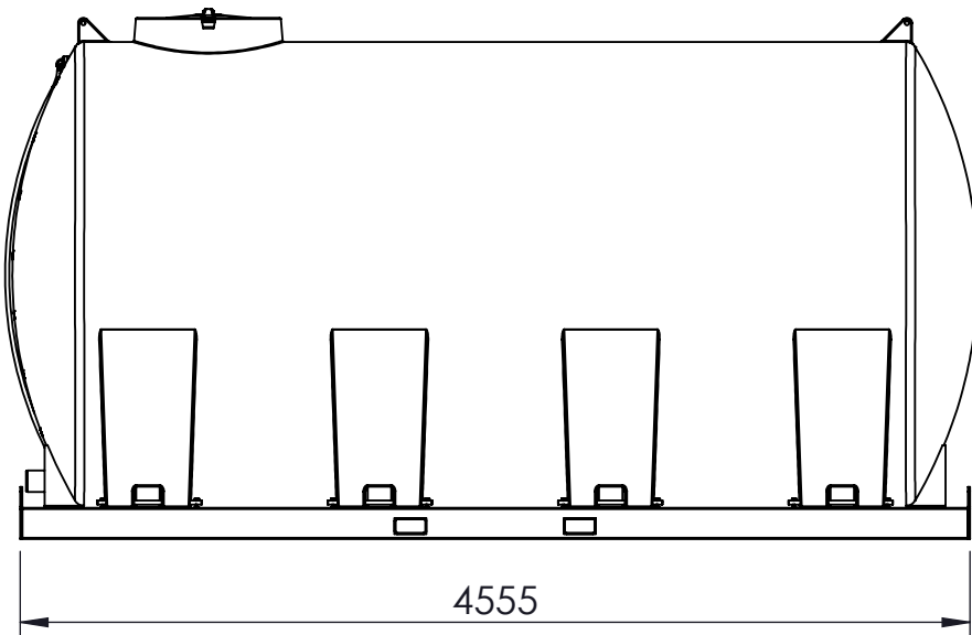
12 O'CLOCK VIEW
