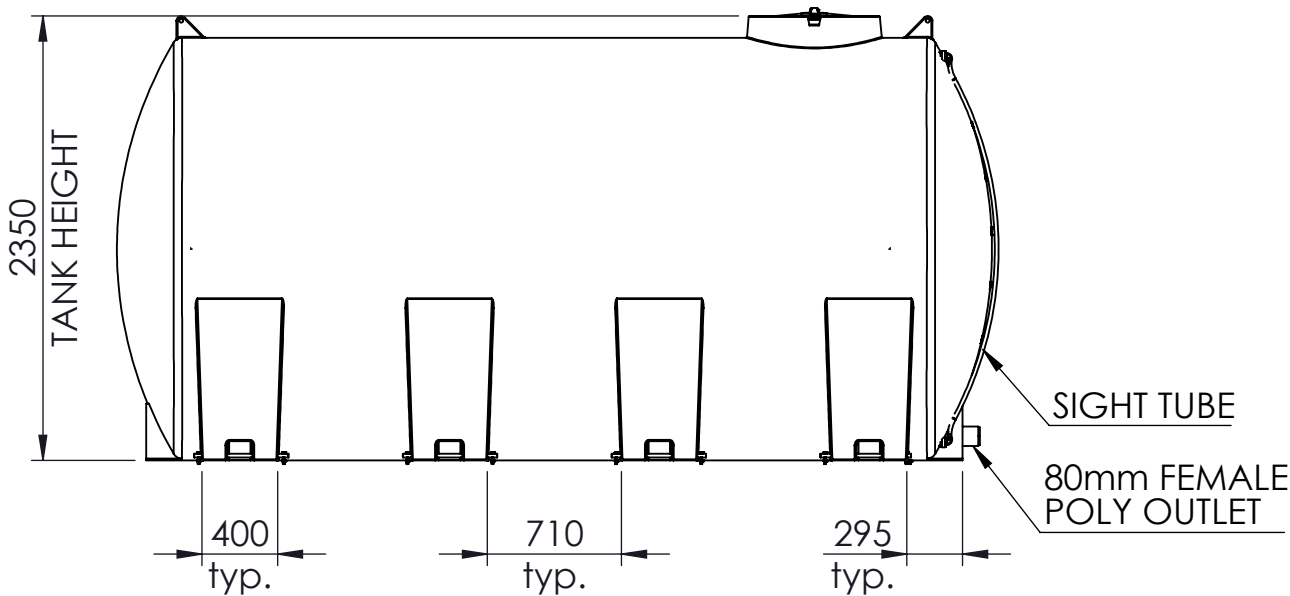
6 O'CLOCK VIEW
