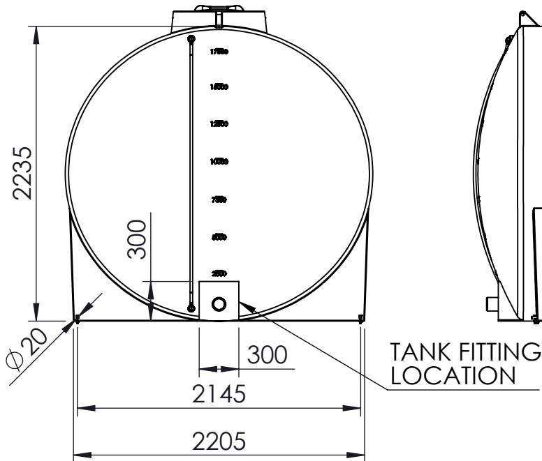
3 O'CLOCK VIEW
