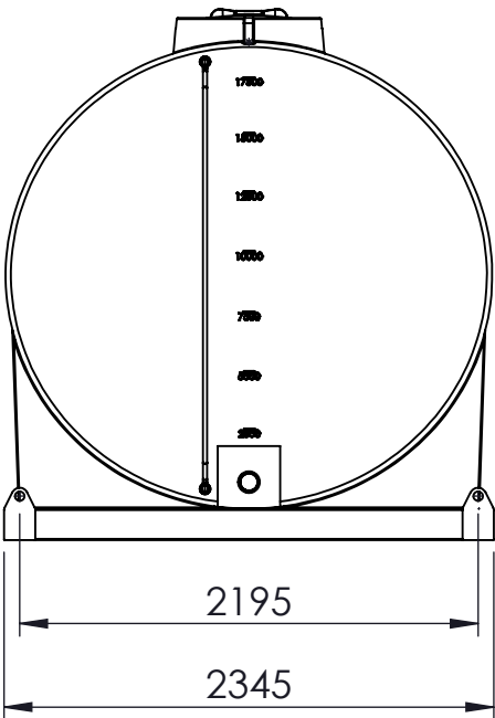
3 O'CLOCK VIEW
