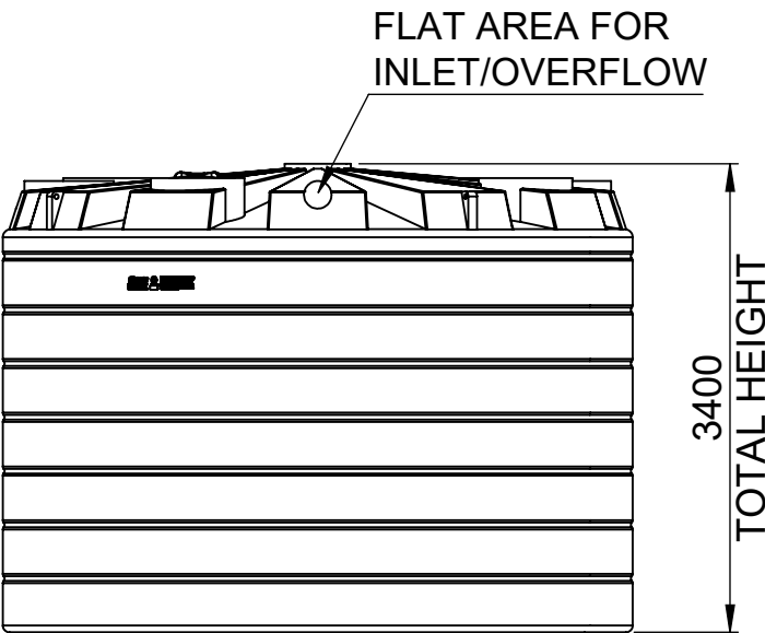
12 O'CLOCK VIEW
