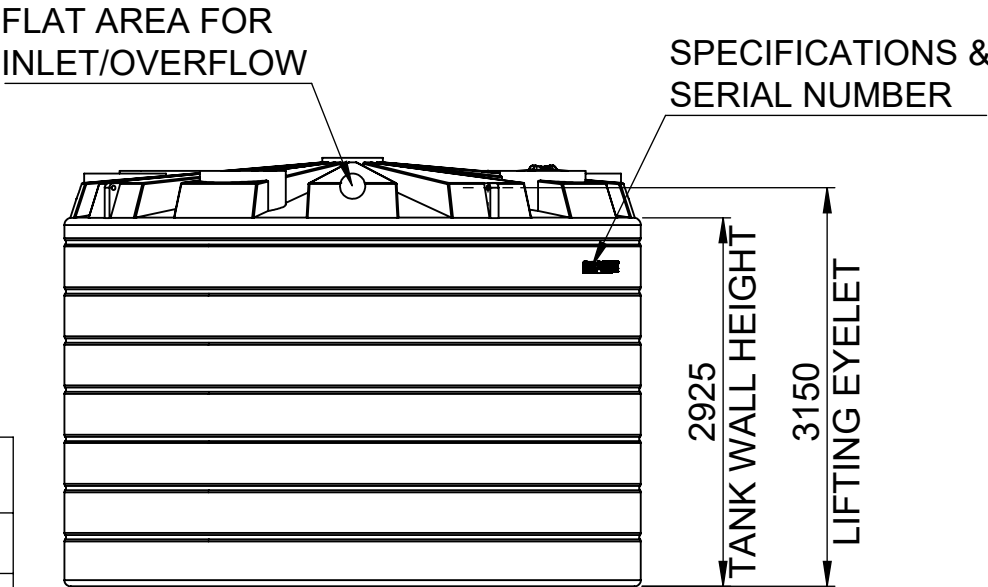
3 O'CLOCK VIEW
