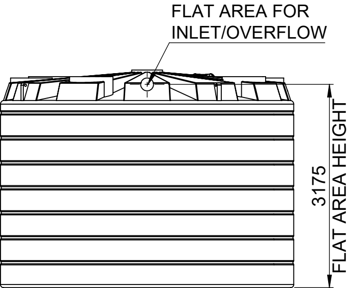
6 O'CLOCK VIEW
