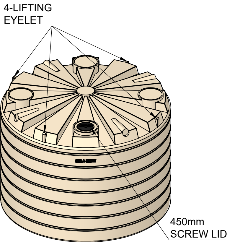
ISOMETRIC VIEW
