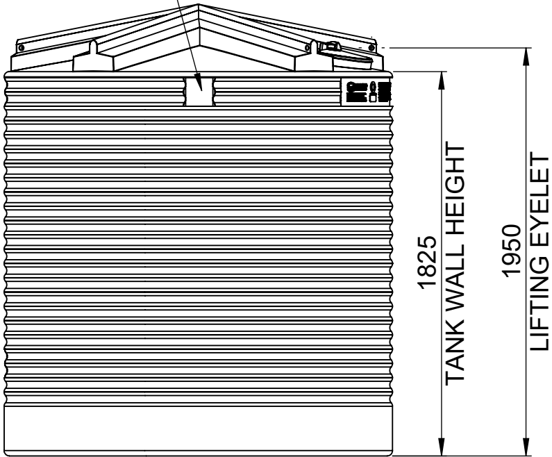
3 O'CLOCK VIEW
