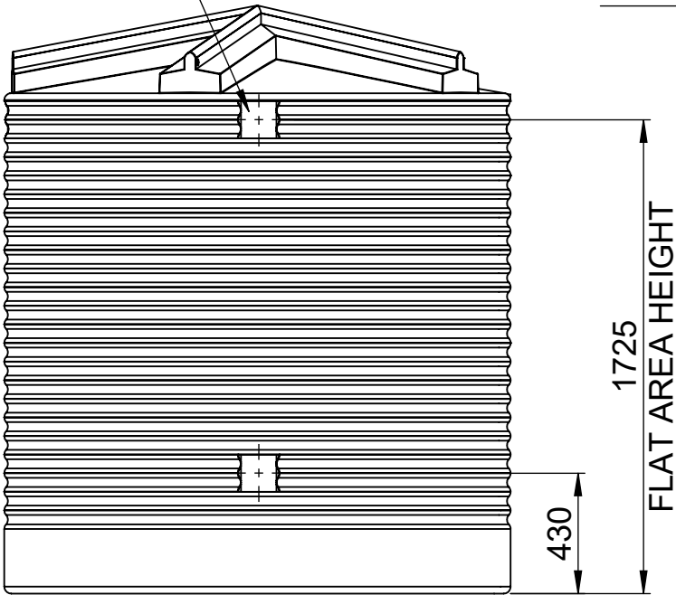
6 O'CLOCK VIEW
