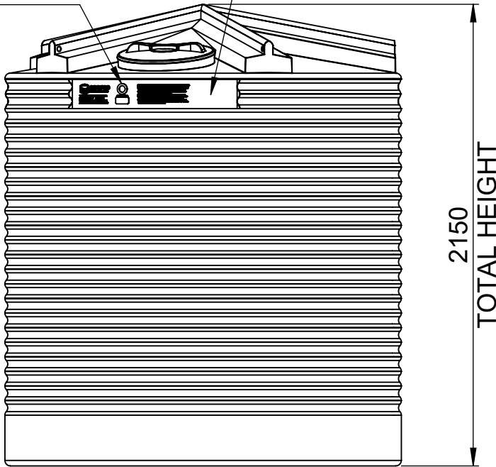
12 O'CLOCK VIEW
