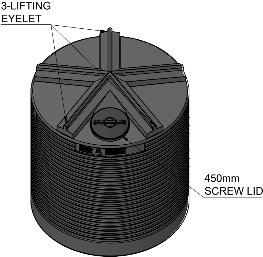
ISOMETRIC VIEW
