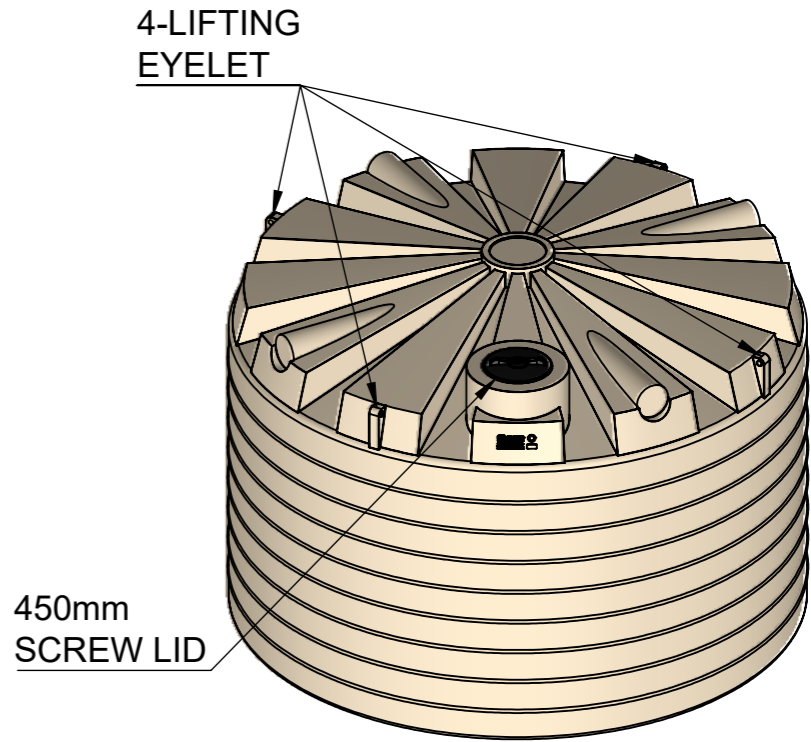
ISOMETRIC VIEW
