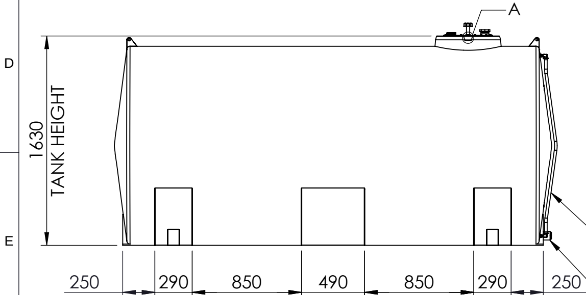
6 O'CLOCK VIEW
