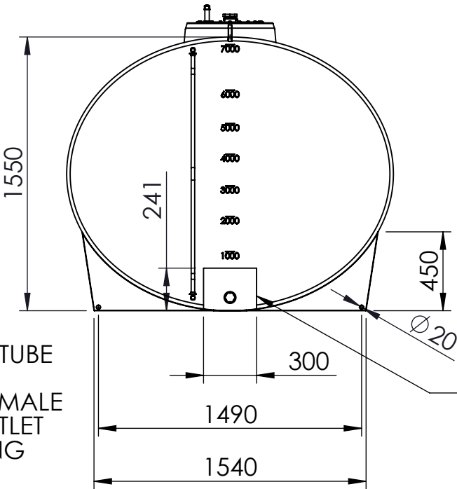
3 O'CLOCK VIEW
