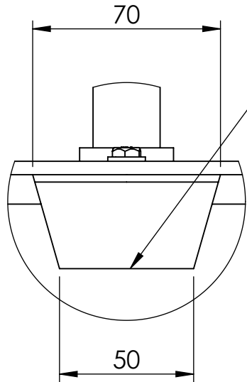
DETAIL A
