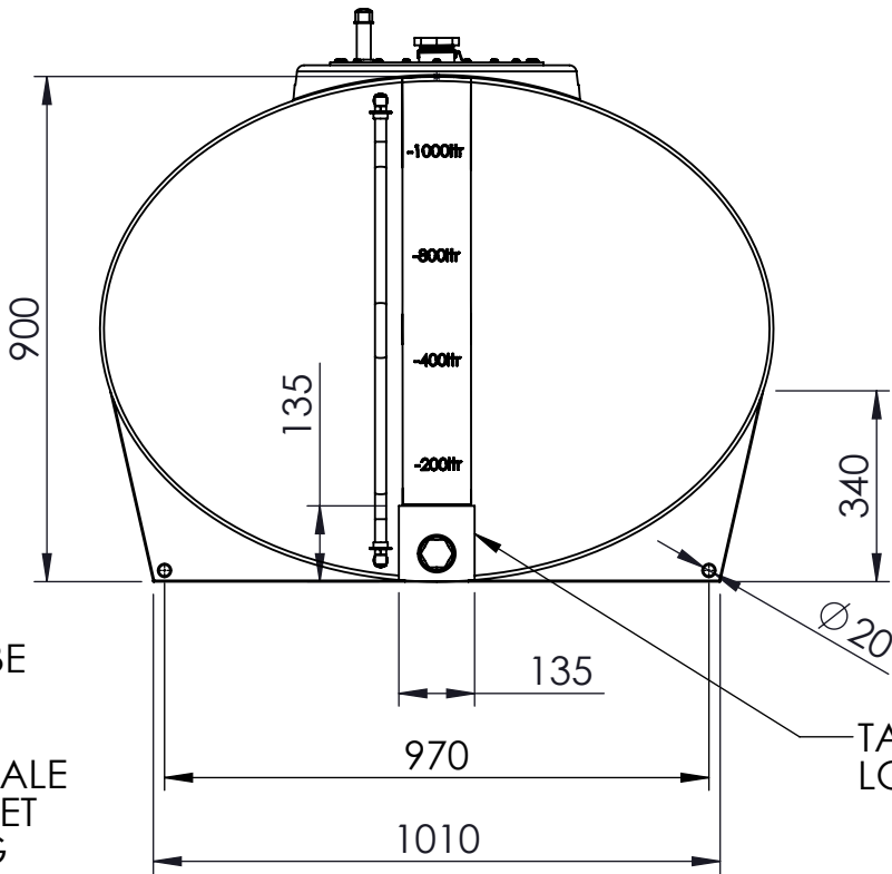
3 O'CLOCK VIEW
