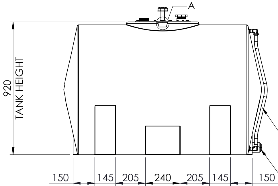
6 O'CLOCK VIEW
